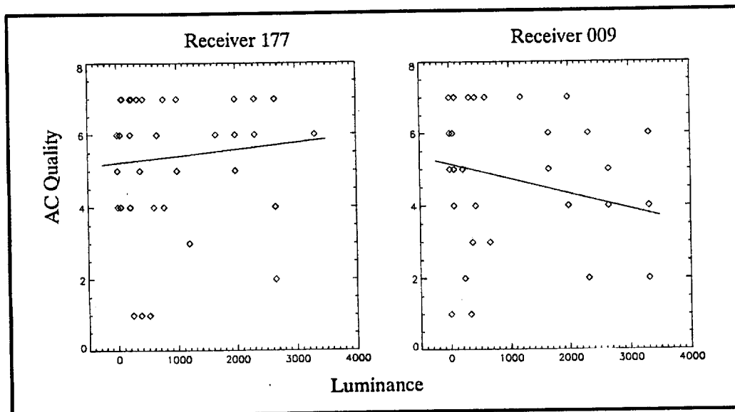
Figure 6. Correlations for the two Significant Receivers.
