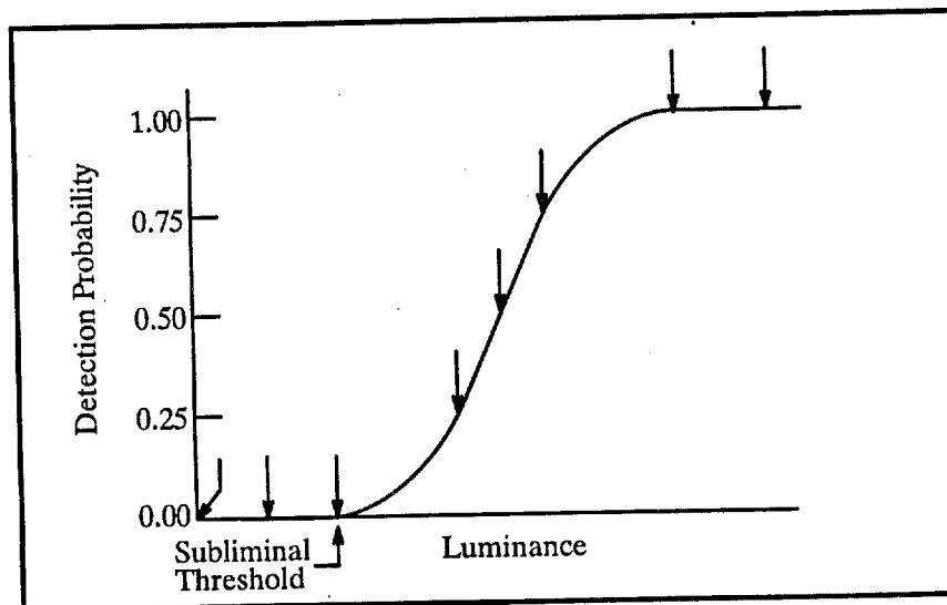
Figure 4. Ideal Psychometric Function
